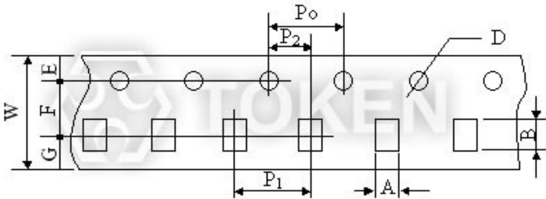
SMD Surface Mount Tape Dimensions
