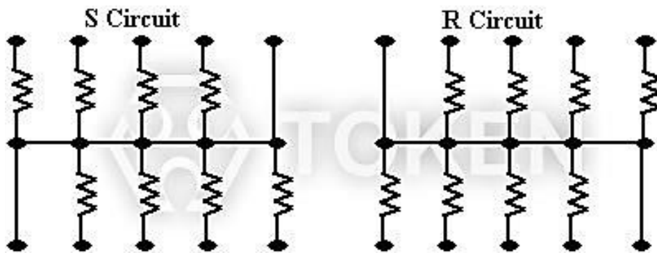
Chip Network (RCN) Circuit
