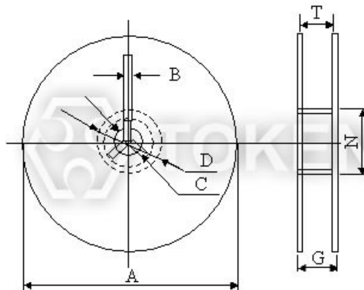
Reel Packaging Dimensions
