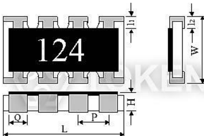
Thick Film Resistor Chip Array (RCA) Dimensions
