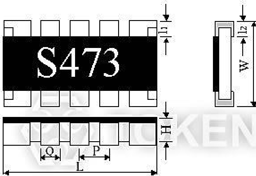
Resistor Chip Networks (RCN) Dimensions
