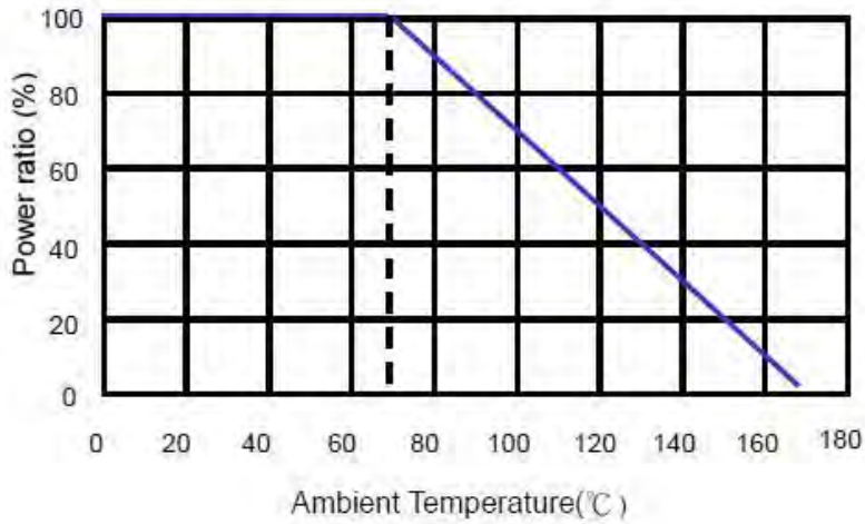
Kelvin Current Sensing Chips (LRF) - Derating Curve
