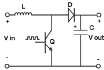
Simplified Boost Regulator
