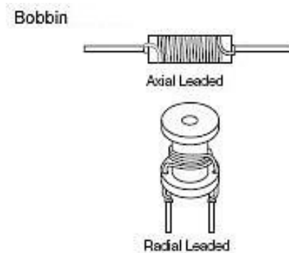
Bobbin Core
