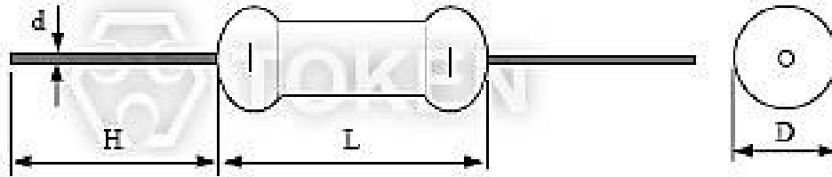
Bulk Ceramic Composition Resistors (RMCC) Dimensions
