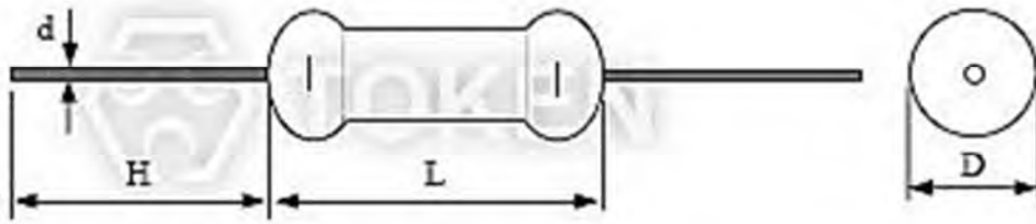
Bulk Ceramic Composition Resistors (RMCC) Dimensions
