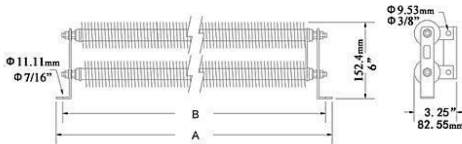
(DRE-G2) Bracket Assembly Options Dimensions
