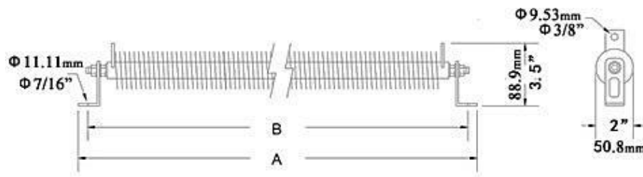
(DRE-G1) Bracket Assembly Options Dimensions
