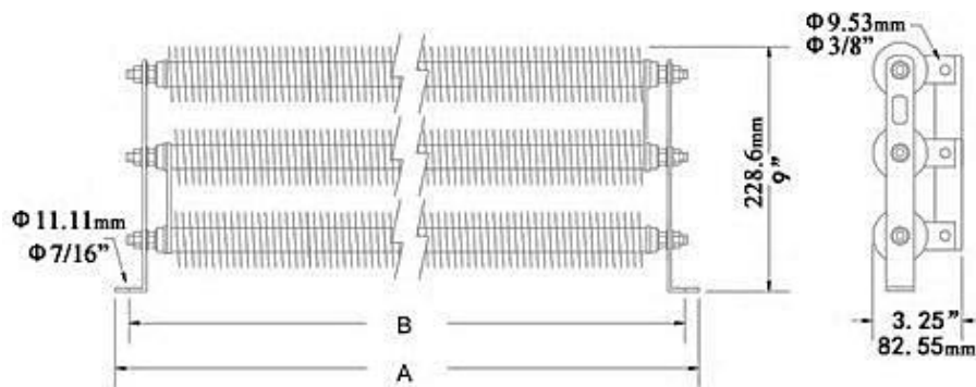
(DRE-G3) Bracket Assembly Options Dimensions
