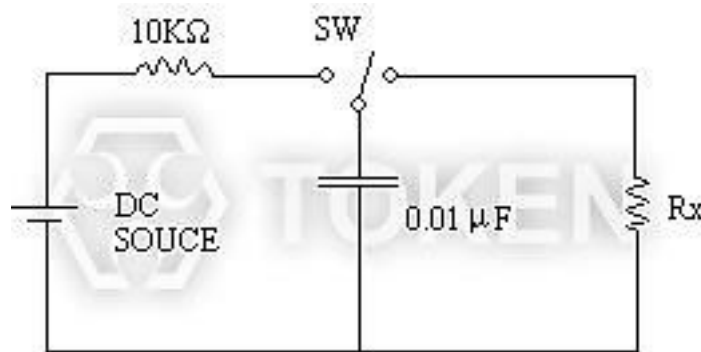
Test Circuit
