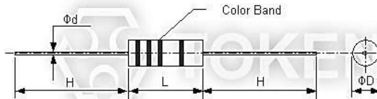
Carbon Composition (CCR) Dimensions (Unit: mm)
