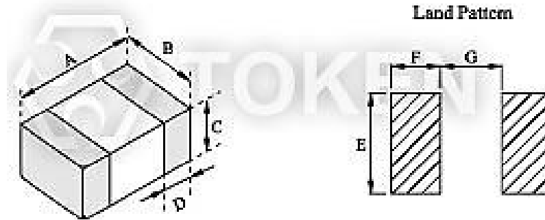
RF Surface Mount (TRMF) Dimensions
