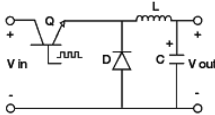
Simplified Buck Regulator
