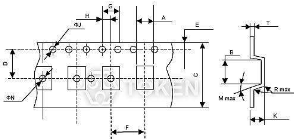
(TA7C/6C/5C/4C) Carrier Tape Dimensions
