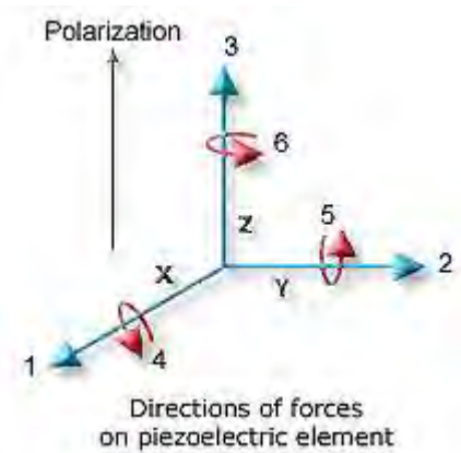
(Figure-1) - Directions of forces on piezoelectric element
