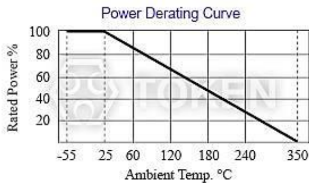
Power (KNP-VE) Derating Curve
