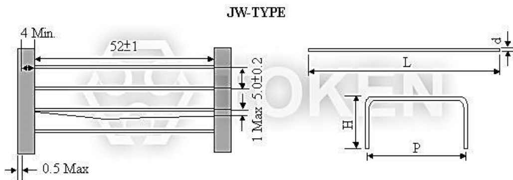
Jumper Wire (JW) Dimensions
