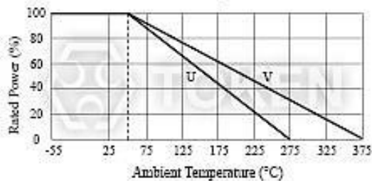
KNP-R Power Derating Curve
