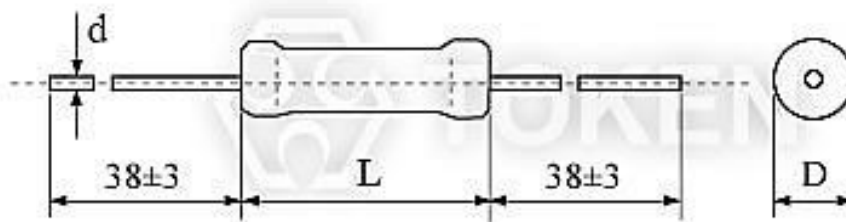
Power Precision Wire Wound Resistor (KNP-R) Dimensions
