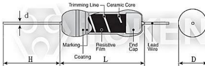
Carbon Film (CF) Dimensions (Unit: mm)
