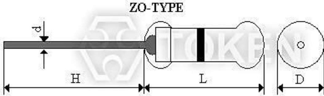
Zero Ohm Resistors (ZO) Dimensions
