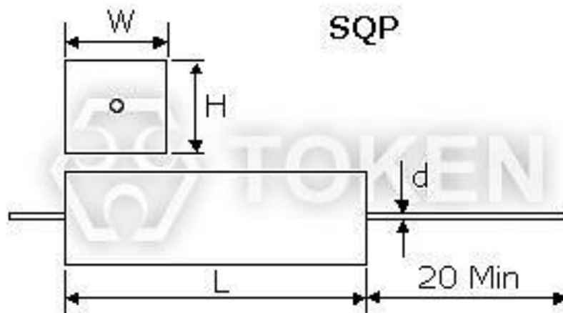
Cement Ceramic Housed (SQP) Dimensions
