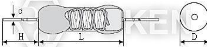
Non-inductive Resistor (KNPN) Dimensions
