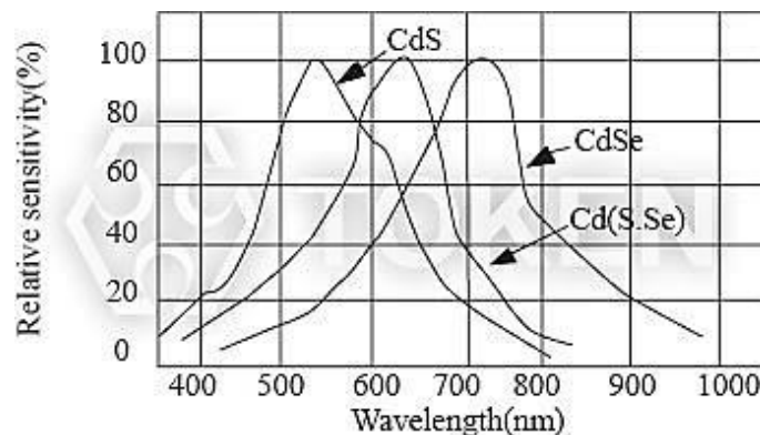
CdS Photoresistors (PGM) Spectral Response
