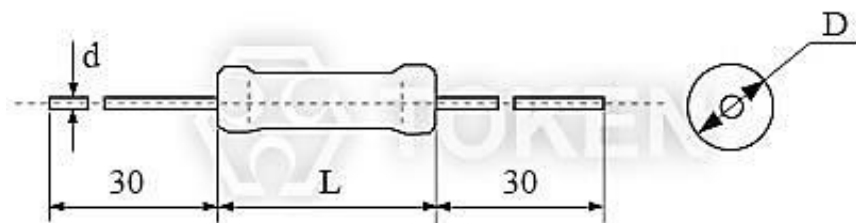
Wire wound Resistors (KNP-VE) Dimensions (Unit: mm)
