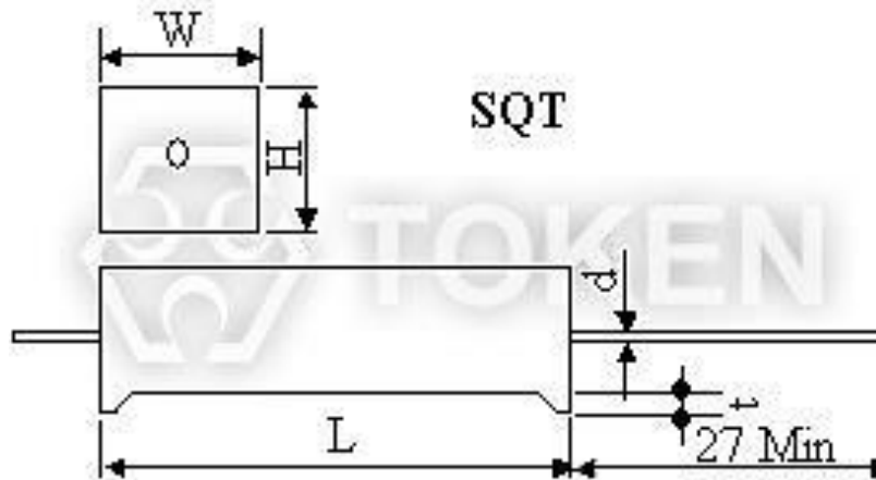
Cement Ceramic Encased (SQT) Dimensions
