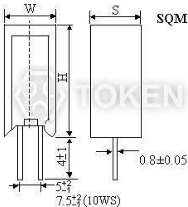
Ceramic Housed (SQM) Dimensions
