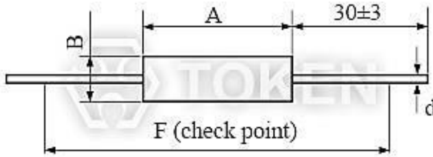
Precision Wire wound (BWW) Dimensions
