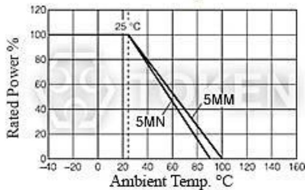
(FKU/FRU) Power Derating Curve
