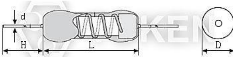
Wirewound Fuse Resistor (FKN) Dimensions (Unit: mm)
