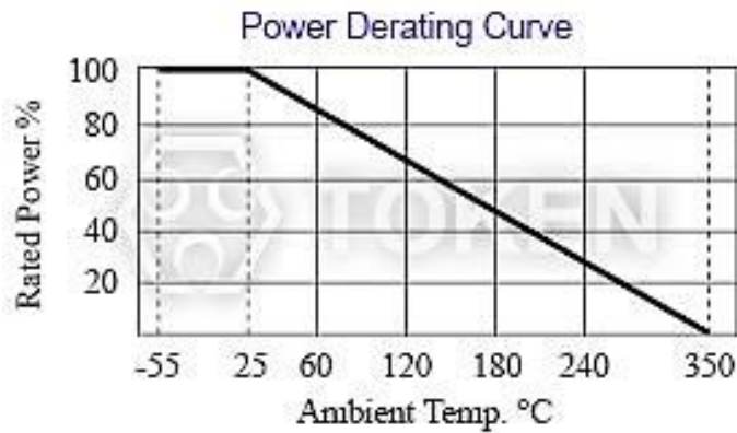
Power (KNP-VE) Derating Curve
