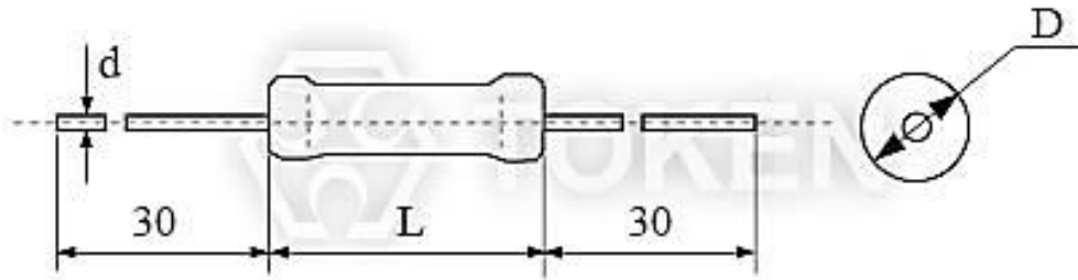
Wire wound Resistors (KNP-VE) Dimensions (Unit: mm)
